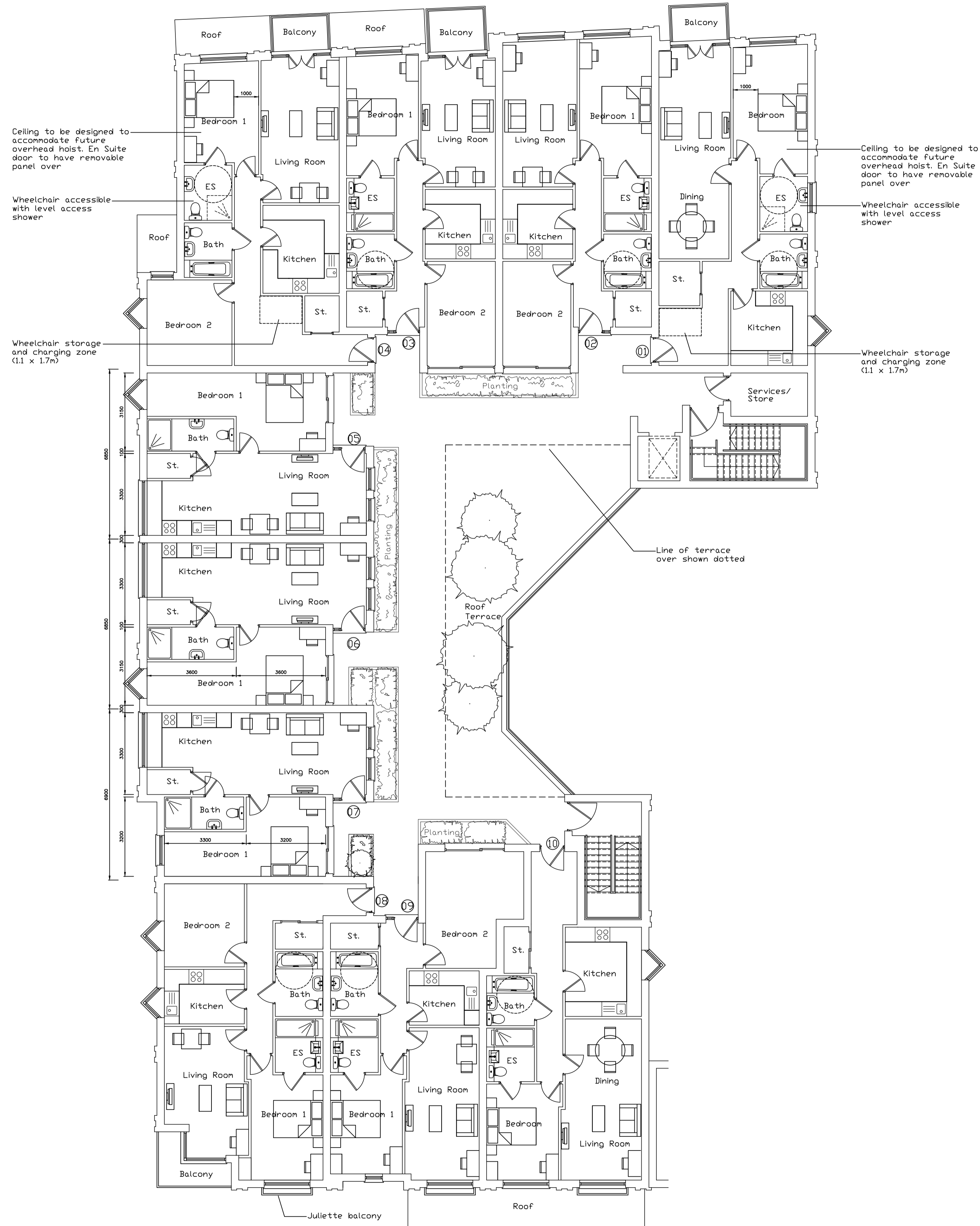
Proposed First Floor Plan Scale 1:100 @ A1
